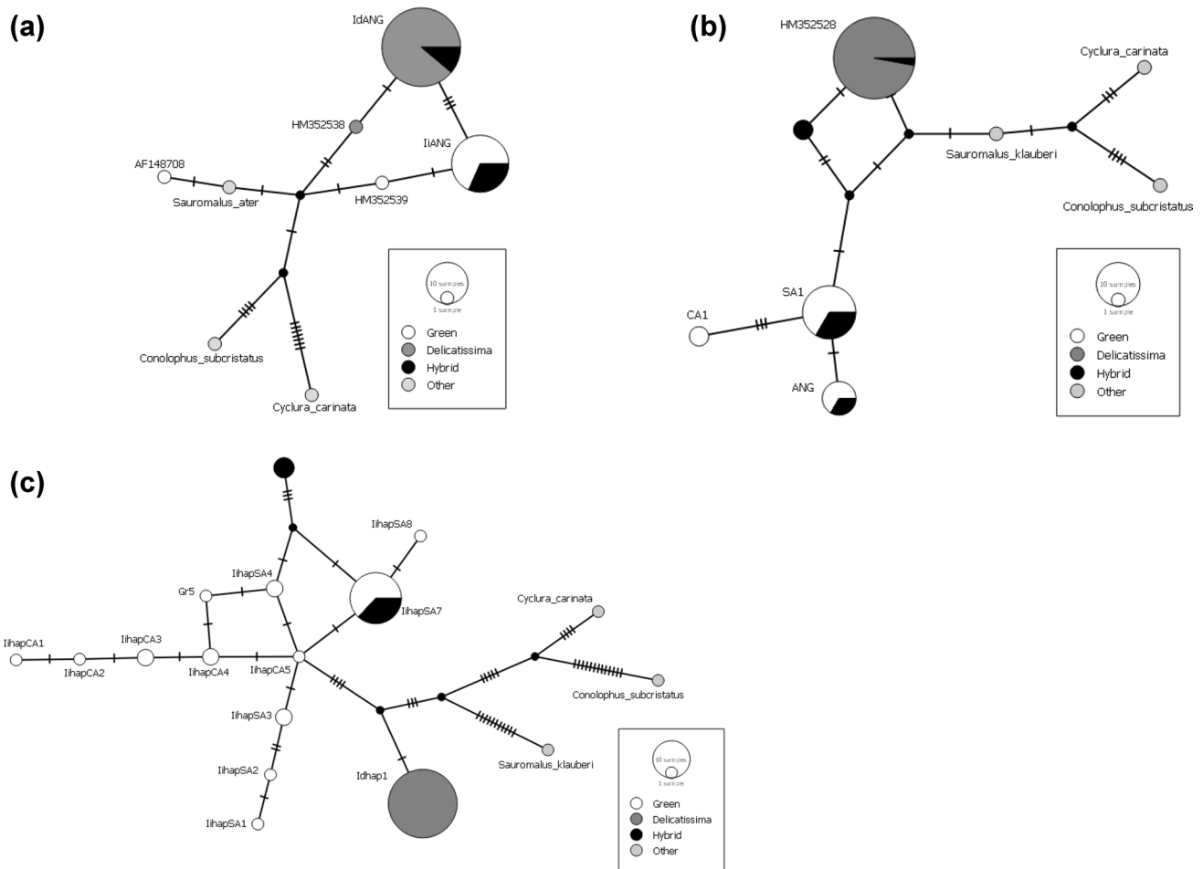
Fig. 5 TCS haplotype networks generated using PopART version 1.7 for the four partial genes isolated in this study, C-mos (a), NT3 (b), PAC (c), and ND4 (d). Each coloured circle represents an individual Iguana haplotype. The size of the circle indicates the relative frequency of sequences belonging to a particular haplotype (smallest circle = 1). Hatch marks along the network branches indicate the number of mutations. Small black circles represent unsampled intermediate haplotypes
